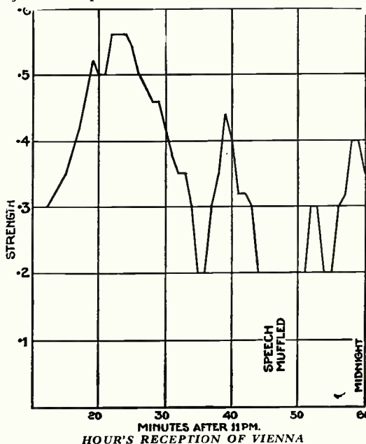
Fig. 2.—Showing a graph of the signal strength from Vienna, which is 900 miles from the receiving station. Quite different from Fecamp's graph shown in Fig. 1!
