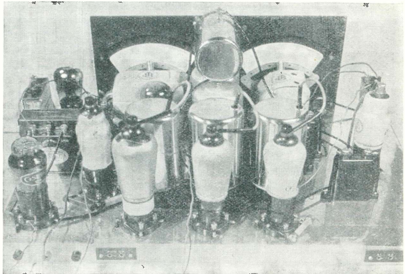
The Modern Super Senior incorporates many of the parts used in the original W. James's design. The set is built on a metal chassis, but there are only a few wires underneath
