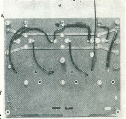
Constructors can easily follow the slight alteration made to the underside wiring of the Lewcos three-coil unit from this photograph
