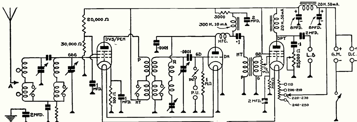
The circuit of the De-luxe D.C. Three is perfectly standard. The valve combination consists of a high-frequency pentode, triode detector and pentode outp. t
