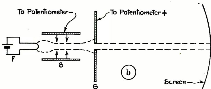
Fig. 2b.—Diagram showing the action of the shield
