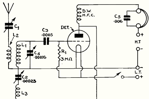
Fig. 1.—A circuit of a simple one-valve short-wave headphone receiver, the construction of which is described in this article
