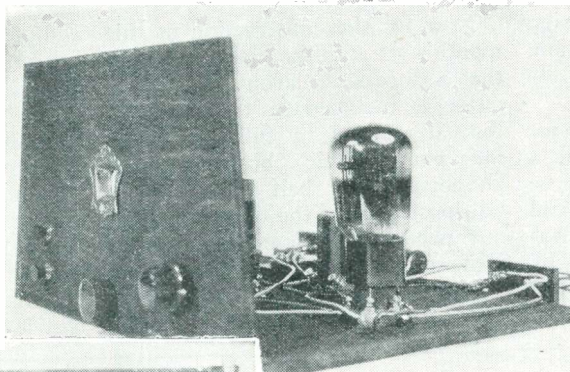
SHOWING THE CONTROLS On the left of the panel is the on-off switch above the wave-change switch; in the centre is the tuner; and on the right is reaction
