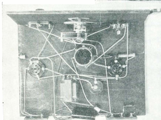
PLAN VIEW OF THE ££ BATTERY TWO This plan view should be used in conjunction with the third-scale wiring plan which appears on page 432. Set building could not be easier
