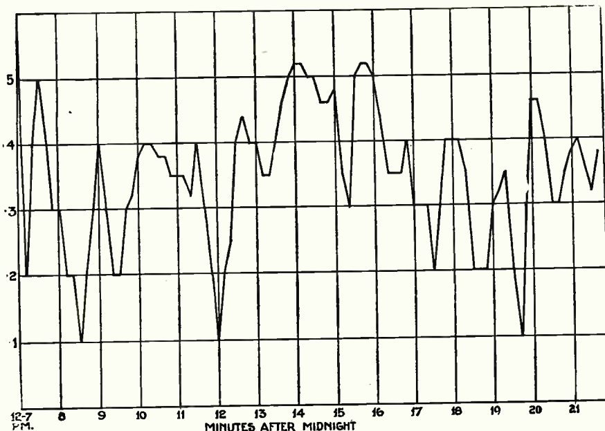
MEASURED STRENGTH OF FECAMP AFTER MIDNIGHT Fig. 1.—Dr. Chapman's graph of the measured signal strength of Radio Normandie between 12.7 and 12.21 a.m. The measurements were made in Devon, about 180 miles from Fecamp
